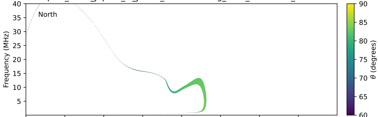
expres_earth_jupiter_io_jrm09_lossc-wid1deg_3kev_20030724_v11.cdf
