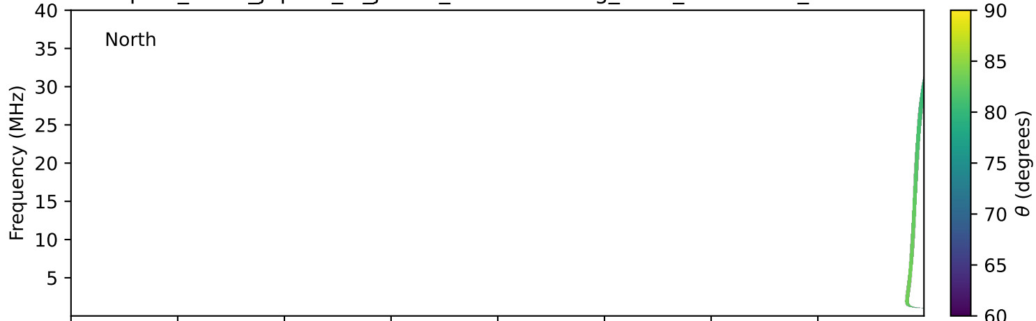
expres_earth_jupiter_io_jrm09_lossc-wid1deg_3kev_20030721_v11.cdf
