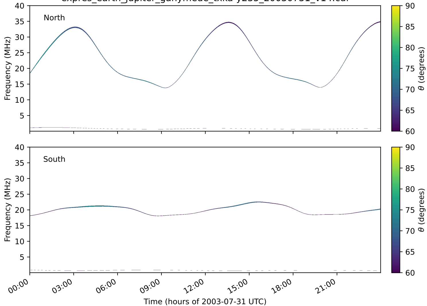
expres_earth_jupiter_ganymede_txka-y235_20030731_v14.cdf
