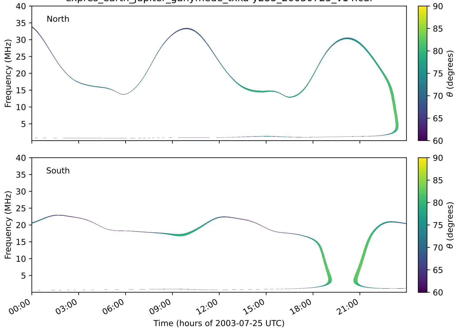
expres_earth_jupiter_ganymede_txka-y235_20030725_v14.cdf
