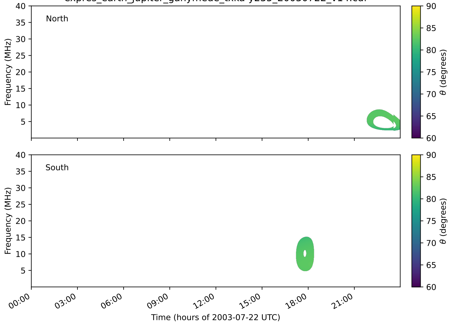
expres_earth_jupiter_ganymede_txka-y235_20030722_v14.cdf
