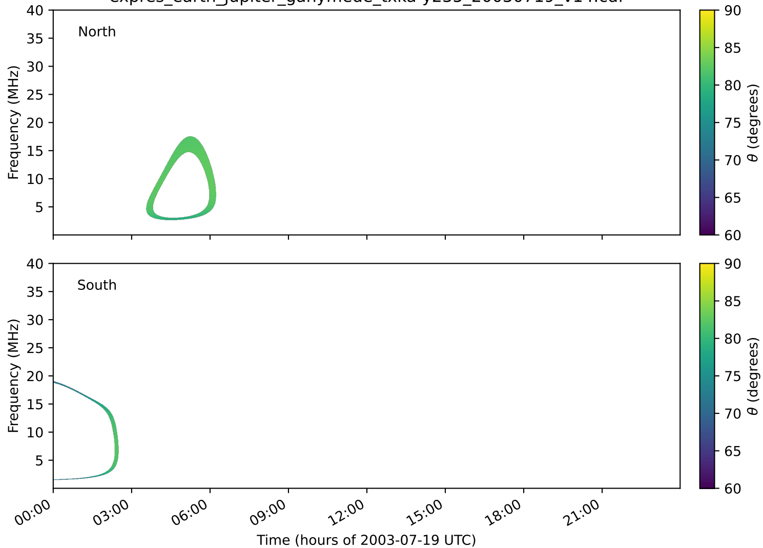
expres_earth_jupiter_ganymede_txka-y235_20030719_v14.cdf
