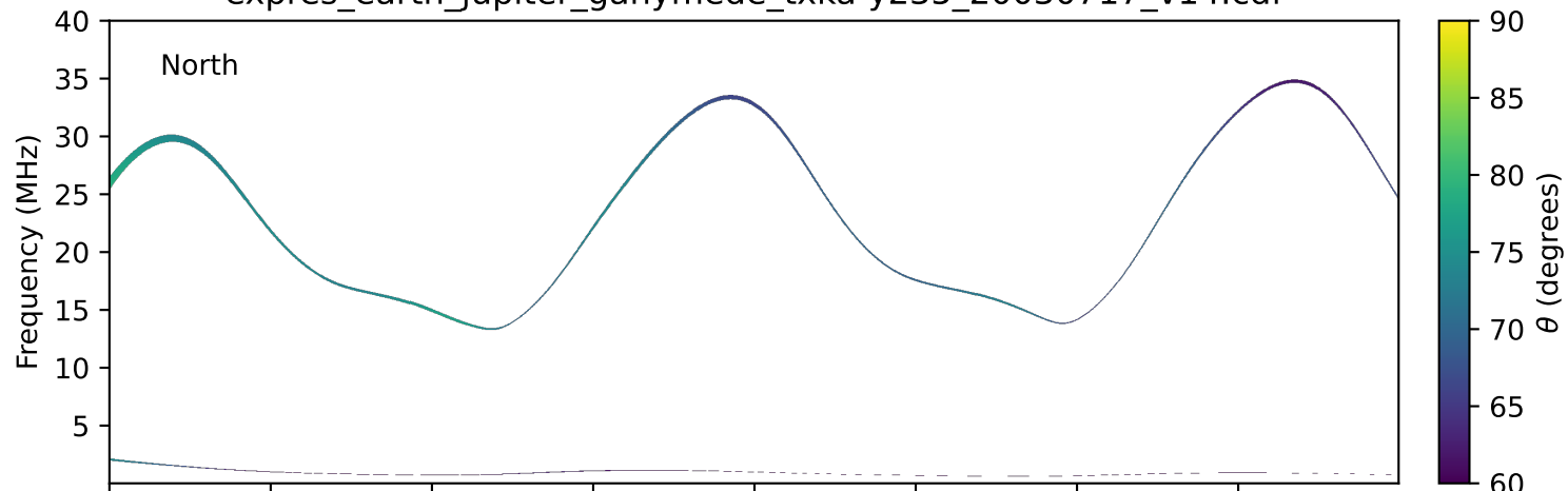
expres_earth_jupiter_ganymede_txka-y235_20030717_v14.cdf
