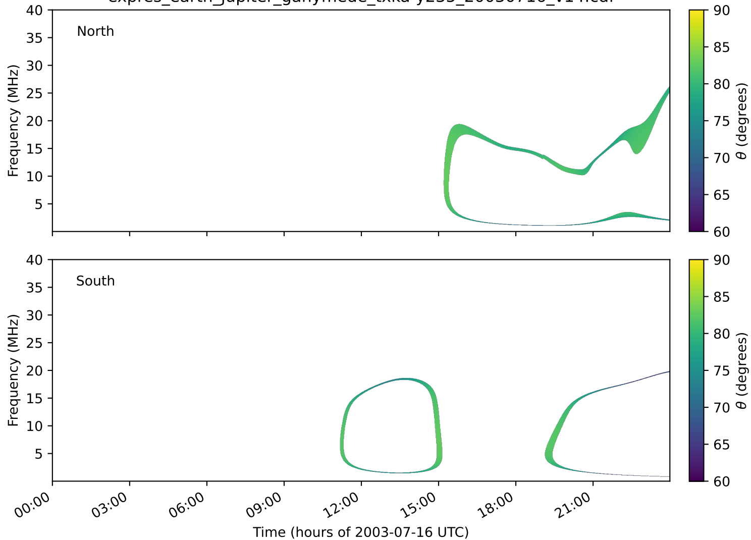
expres_earth_jupiter_ganymede_txka-y235_20030716_v14.cdf
