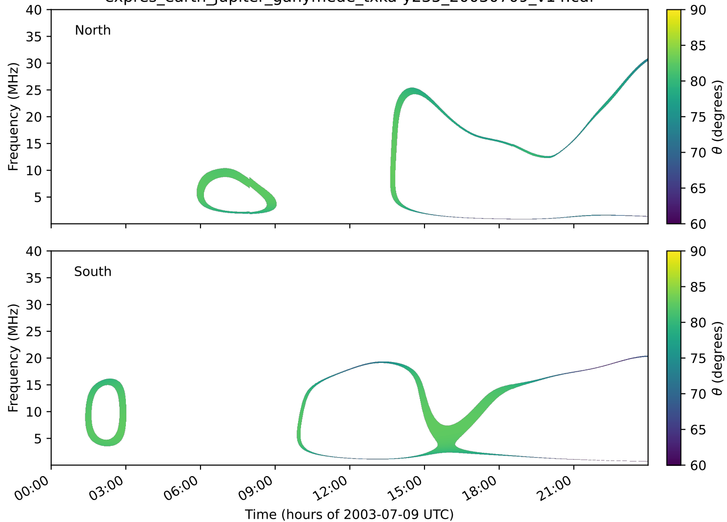
expres_earth_jupiter_ganymede_txka-y235_20030709_v14.cdf
