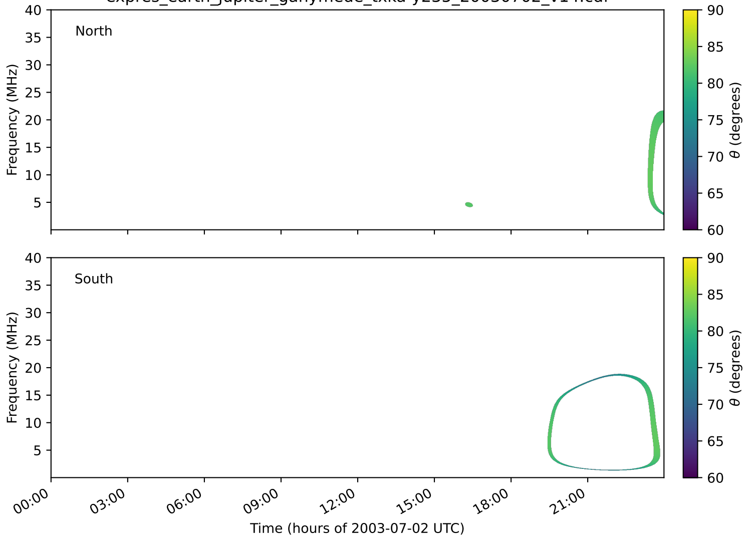
expres_earth_jupiter_ganymede_txka-y235_20030702_v14.cdf
