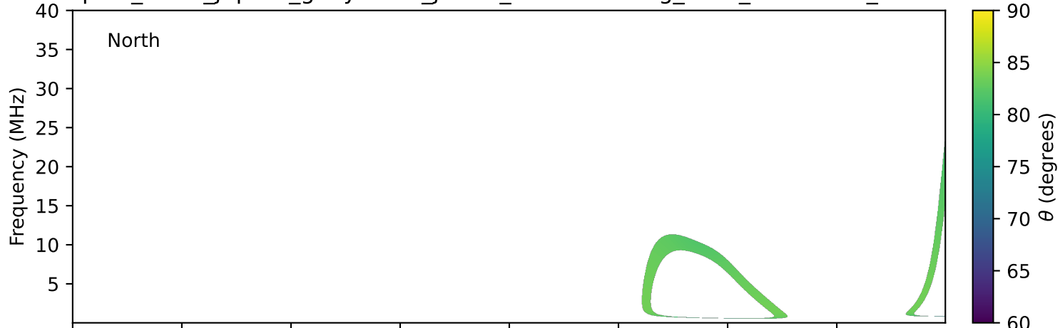
expres_earth_jupiter_ganymede_jrm33_lossc-wid1deg_3kev_20030716_v11.cdf
