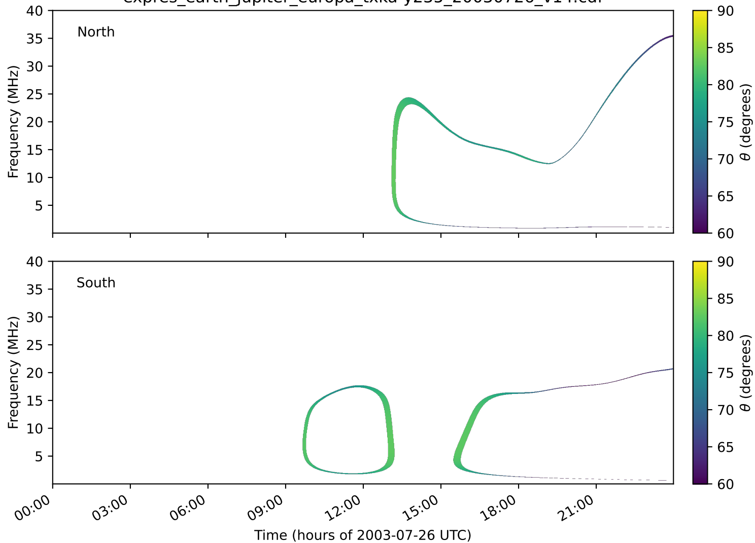
expres_earth_jupiter_europa_txka-y235_20030726_v14.cdf
