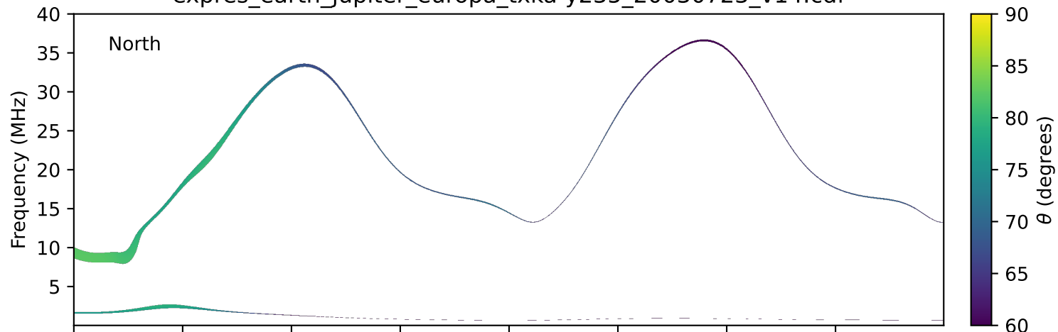
expres_earth_jupiter_europa_txka-y235_20030723_v14.cdf
