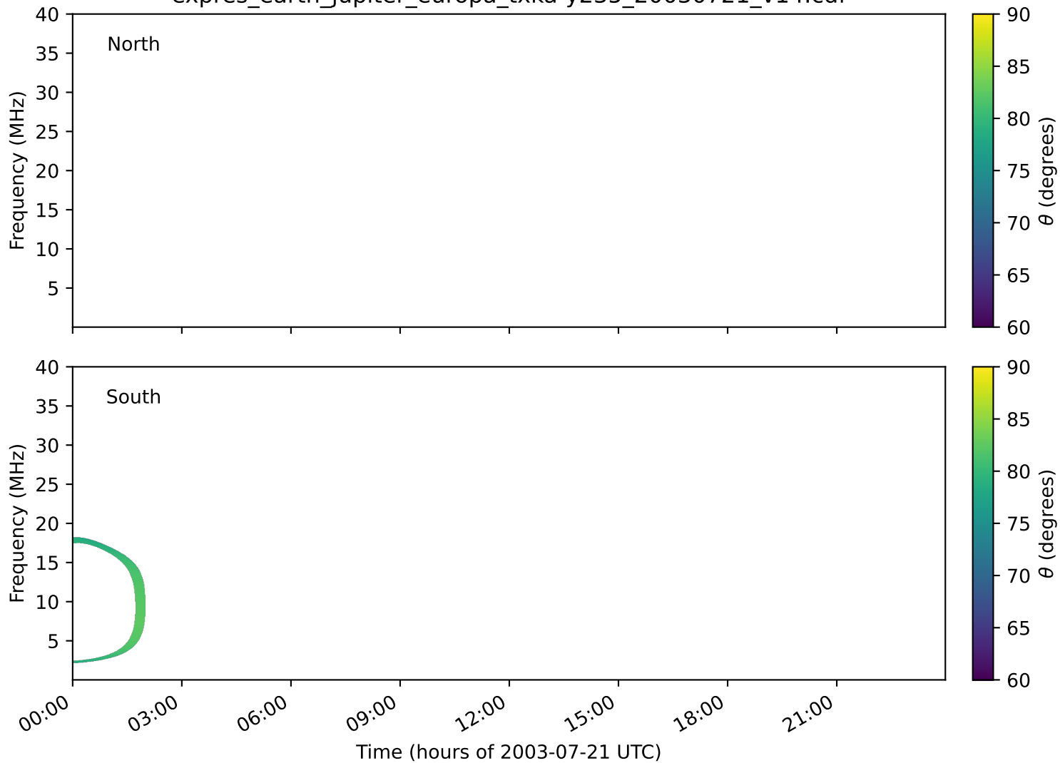
expres_earth_jupiter_europa_txka-y235_20030721_v14.cdf
