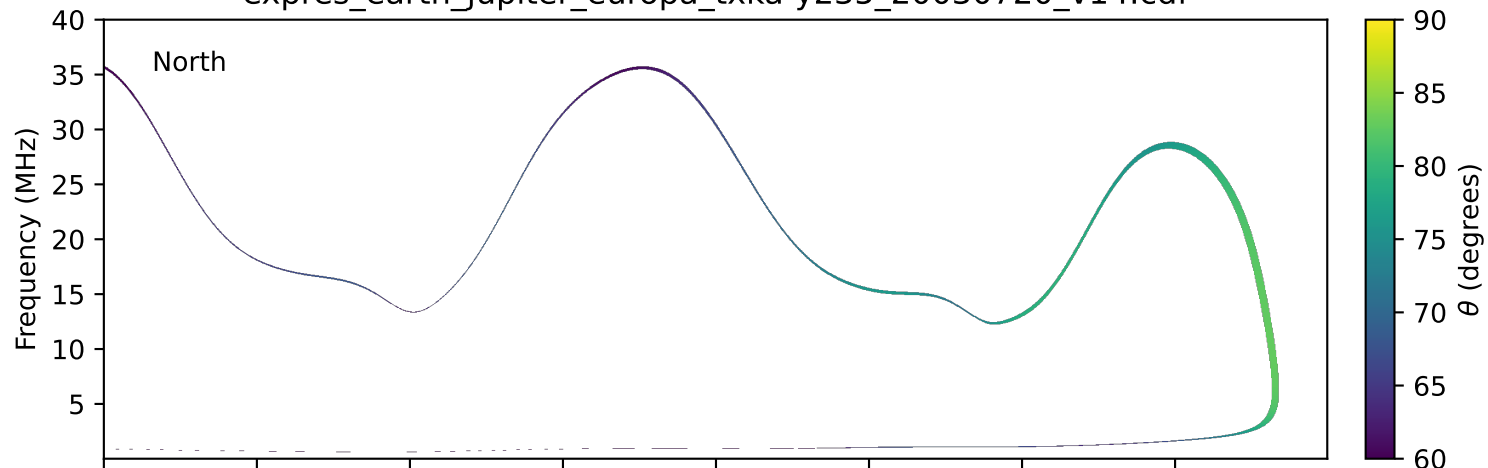
expres_earth_jupiter_europa_txka-y235_20030720_v14.cdf
