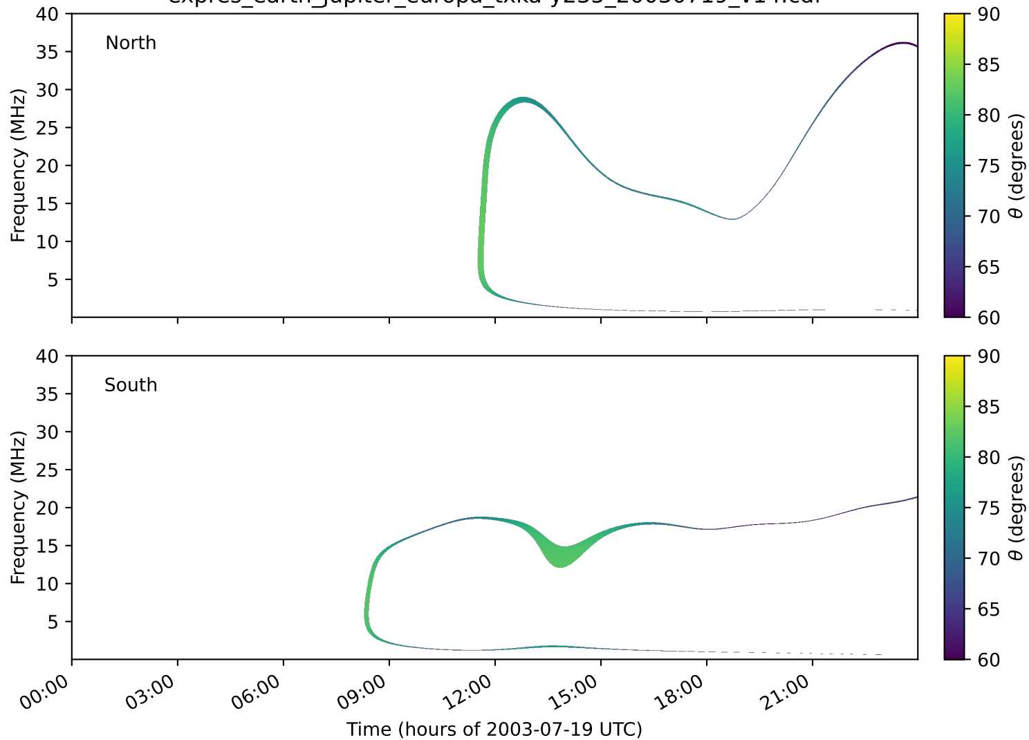
expres_earth_jupiter_europa_txka-y235_20030719_v14.cdf
