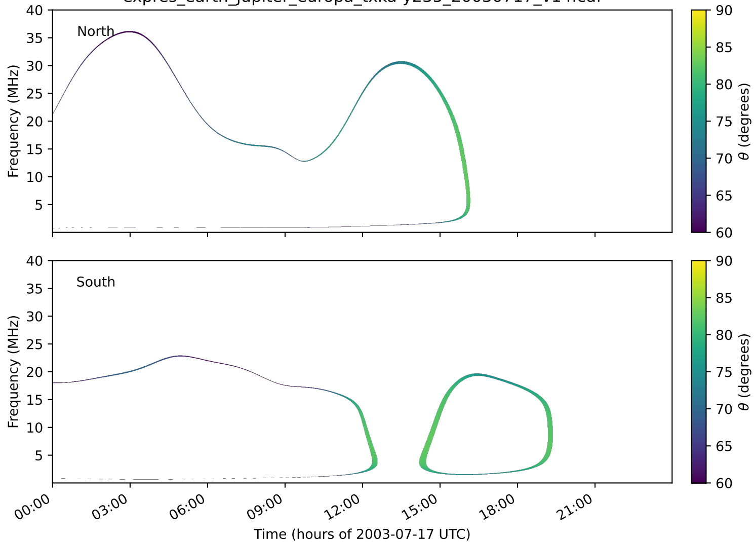
expres_earth_jupiter_europa_txka-y235_20030717_v14.cdf
