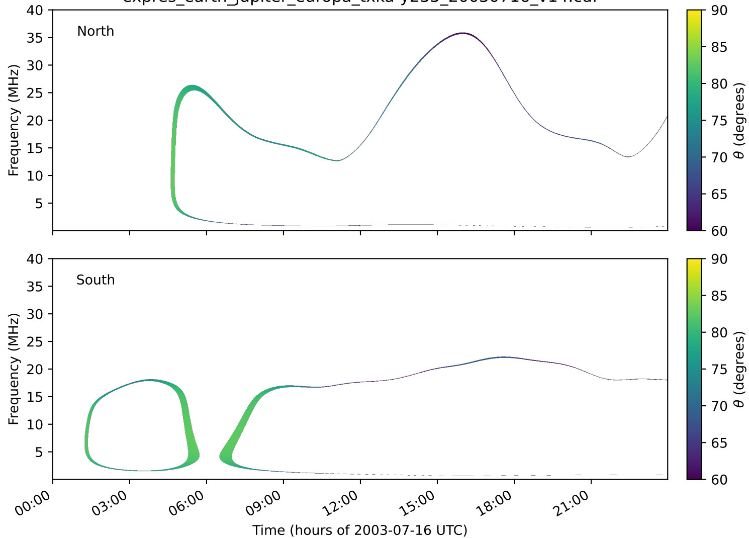
expres_earth_jupiter_europa_txka-y235_20030716_v14.cdf
