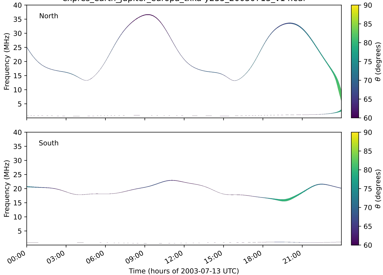
expres_earth_jupiter_europa_txka-y235_20030713_v14.cdf
