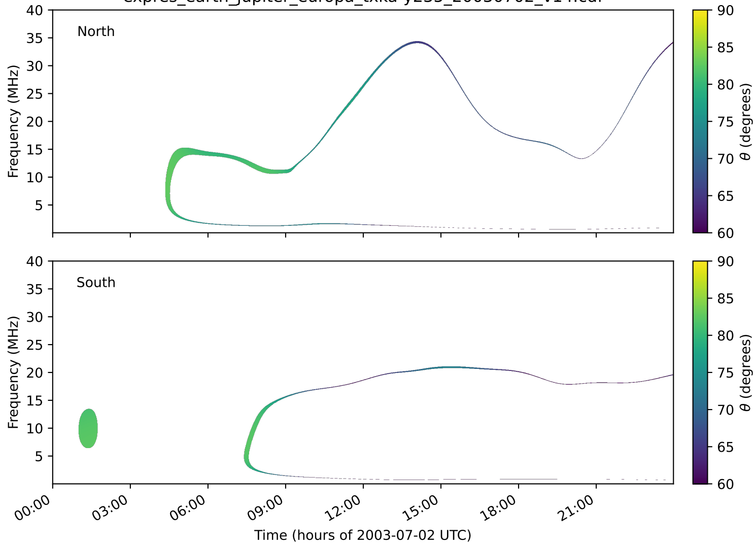
expres_earth_jupiter_europa_txka-y235_20030702_v14.cdf
