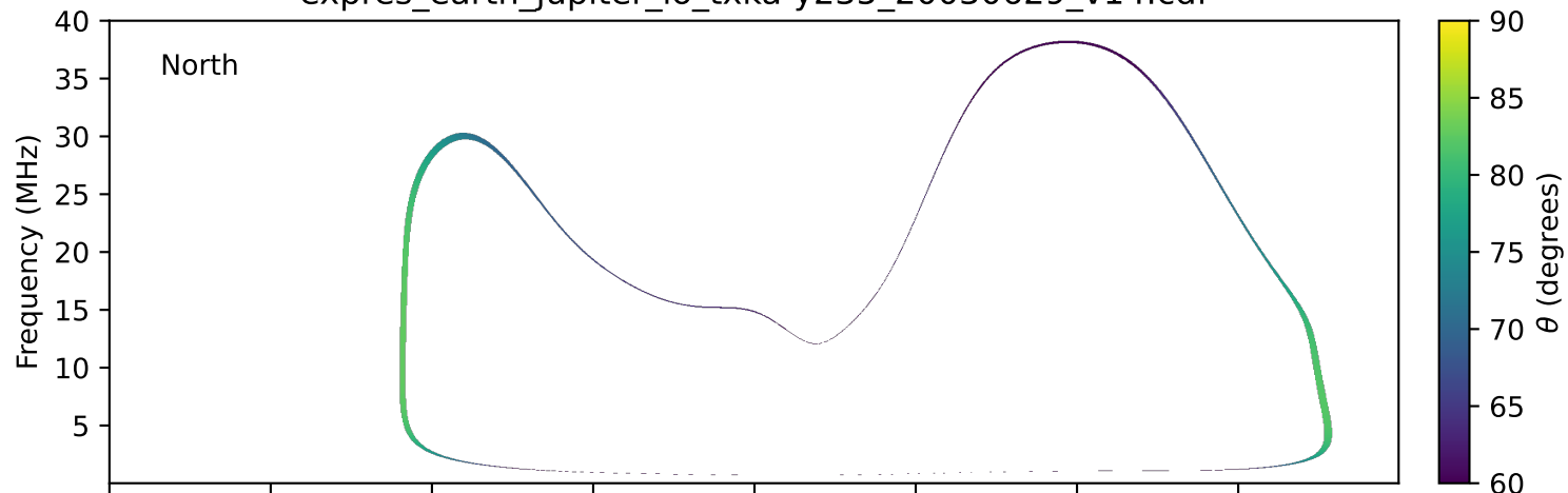
expres_earth_jupiter_io_txka-y235_20030629_v14.cdf
