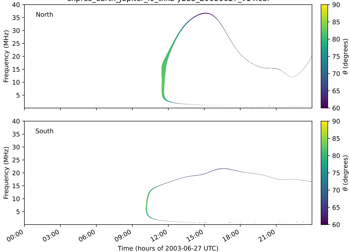
expres_earth_jupiter_io_txka-y235_20030627_v14.cdf
