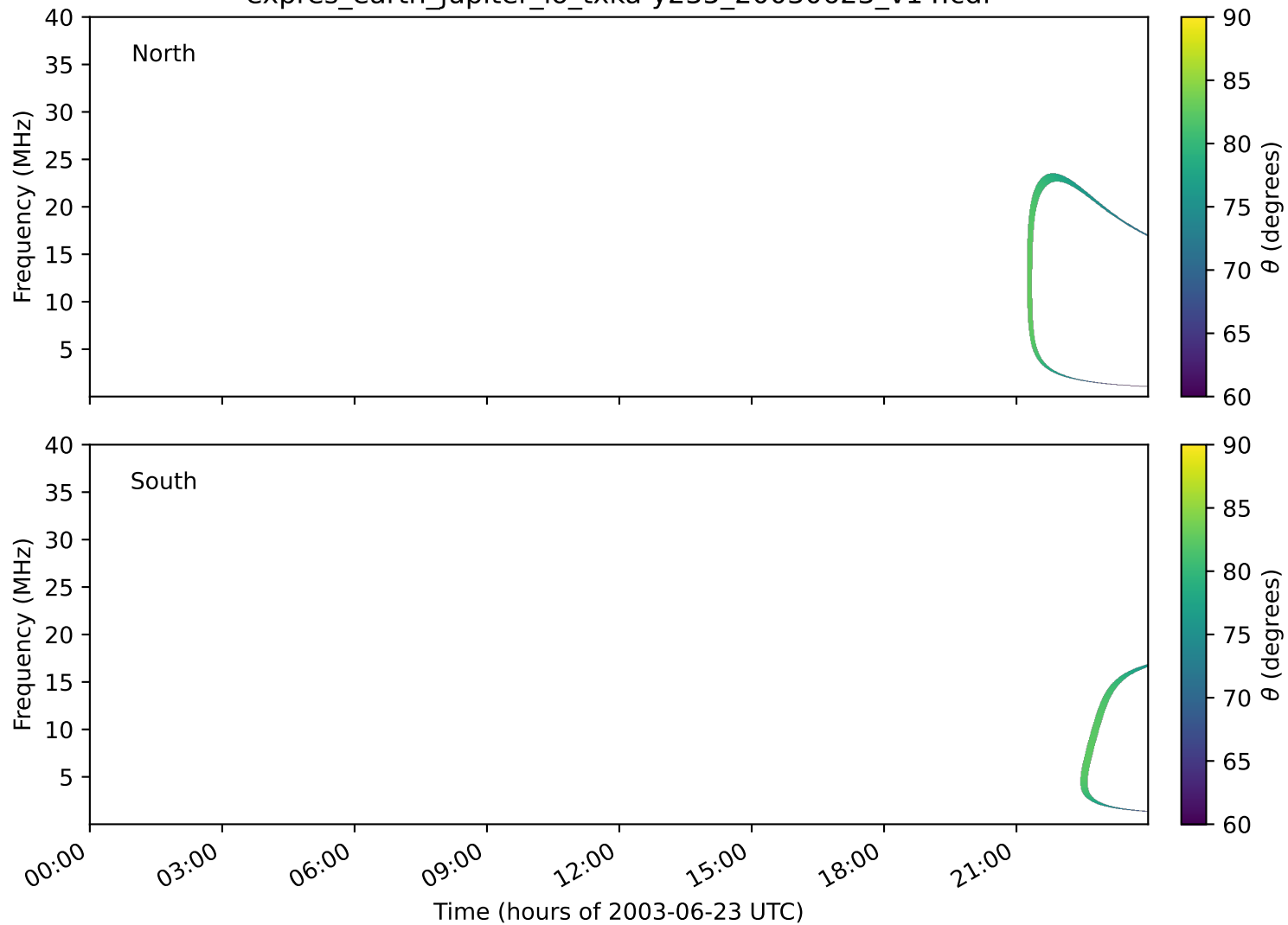
expres_earth_jupiter_io_txka-y235_20030623_v14.cdf
