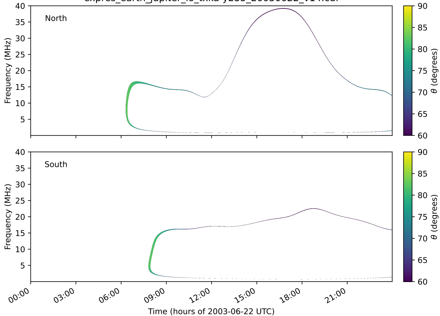
expres_earth_jupiter_io_txka-y235_20030622_v14.cdf
