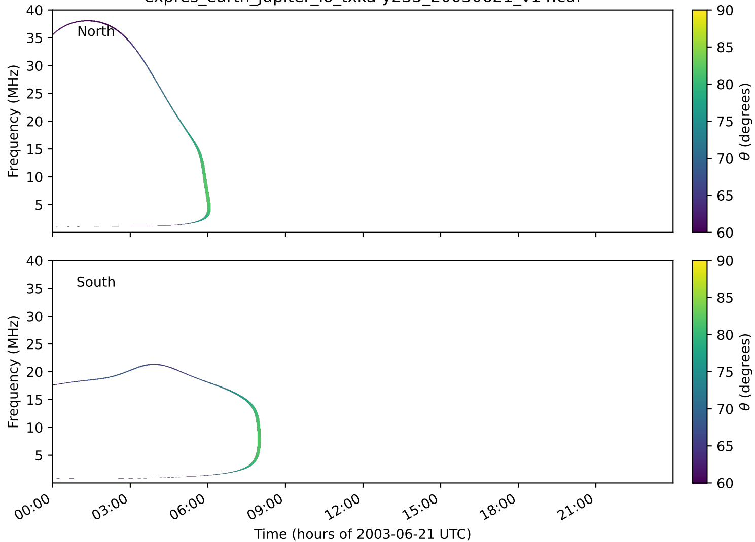
expres_earth_jupiter_io_txka-y235_20030621_v14.cdf
