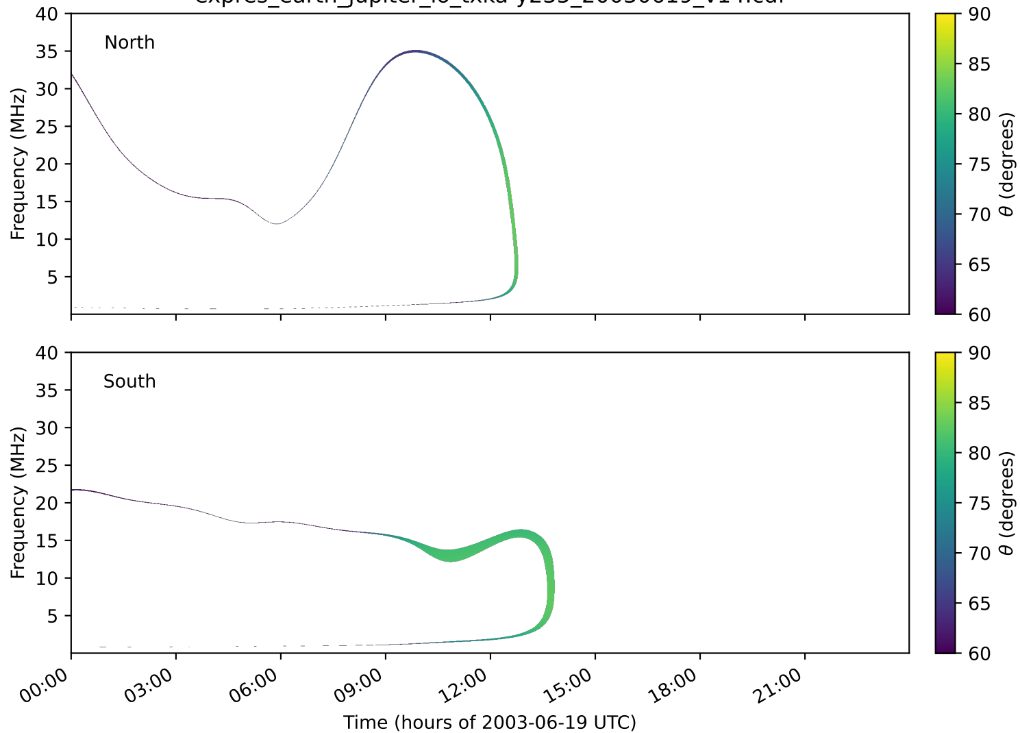
expres_earth_jupiter_io_txka-y235_20030619_v14.cdf
