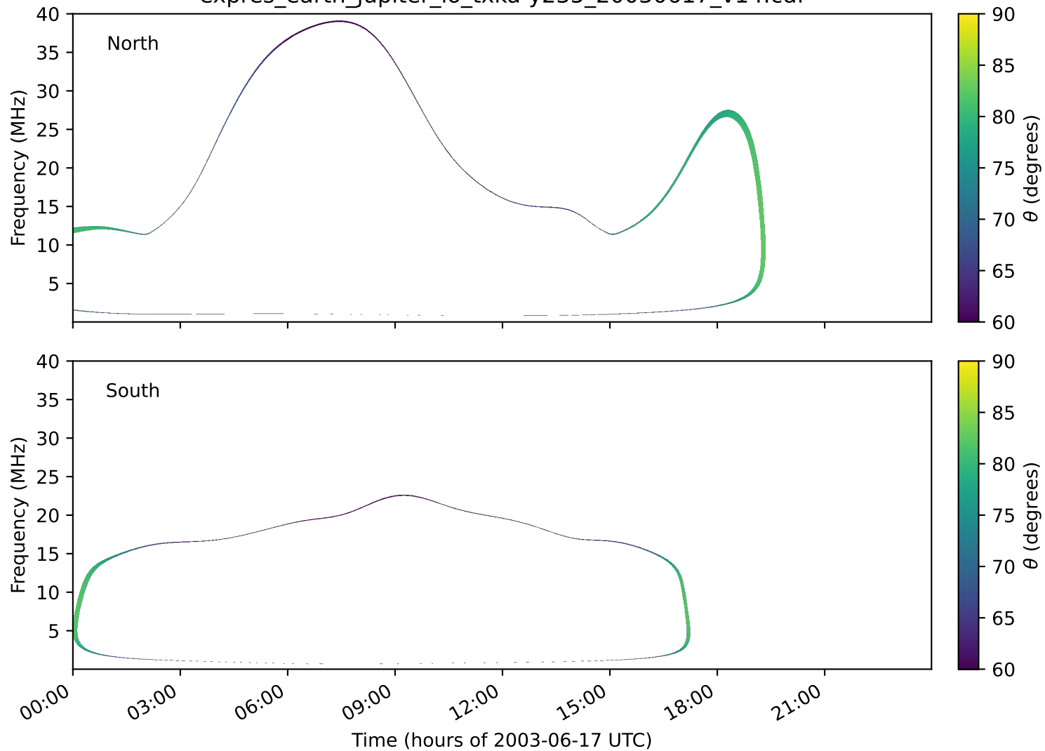
expres_earth_jupiter_io_txka-y235_20030617_v14.cdf
