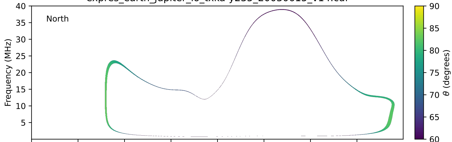
expres_earth_jupiter_io_txka-y235_20030615_v14.cdf
