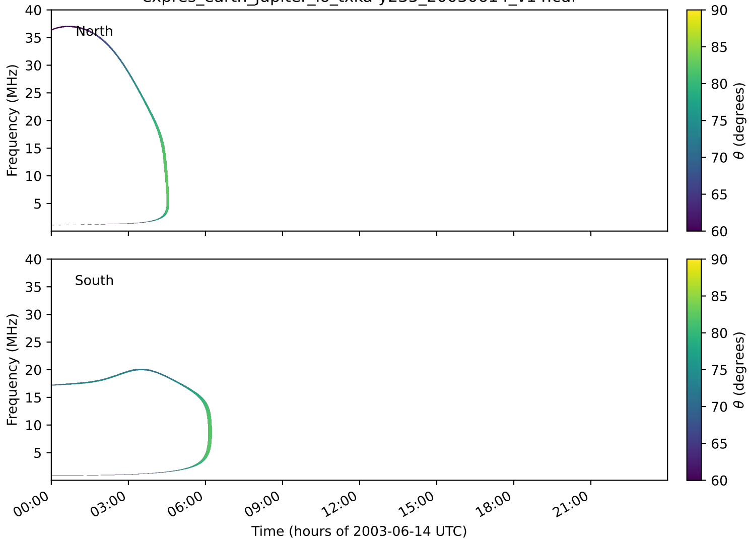
expres_earth_jupiter_io_txka-y235_20030614_v14.cdf
