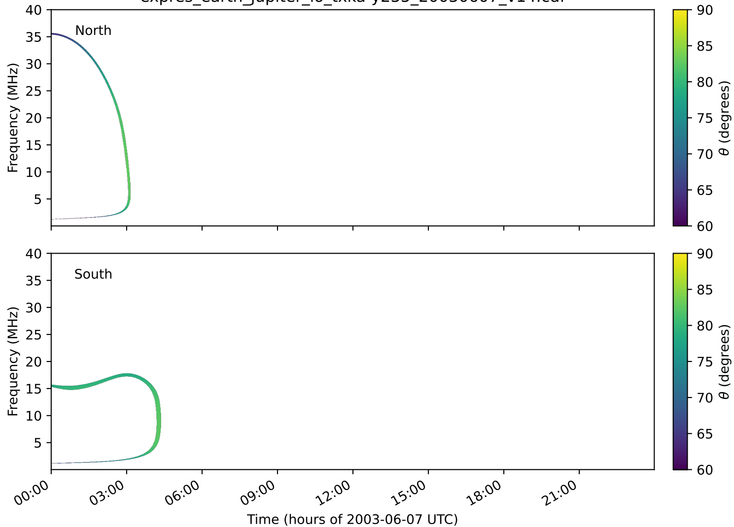
expres_earth_jupiter_io_txka-y235_20030607_v14.cdf
