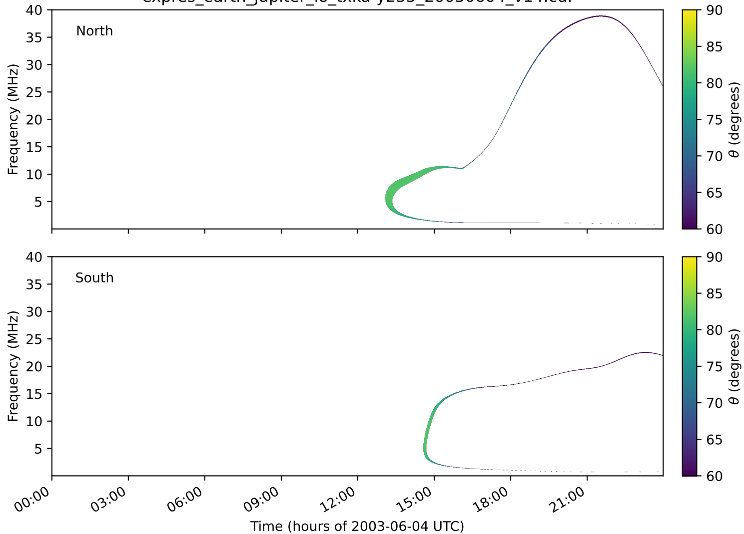
expres_earth_jupiter_io_txka-y235_20030604_v14.cdf
