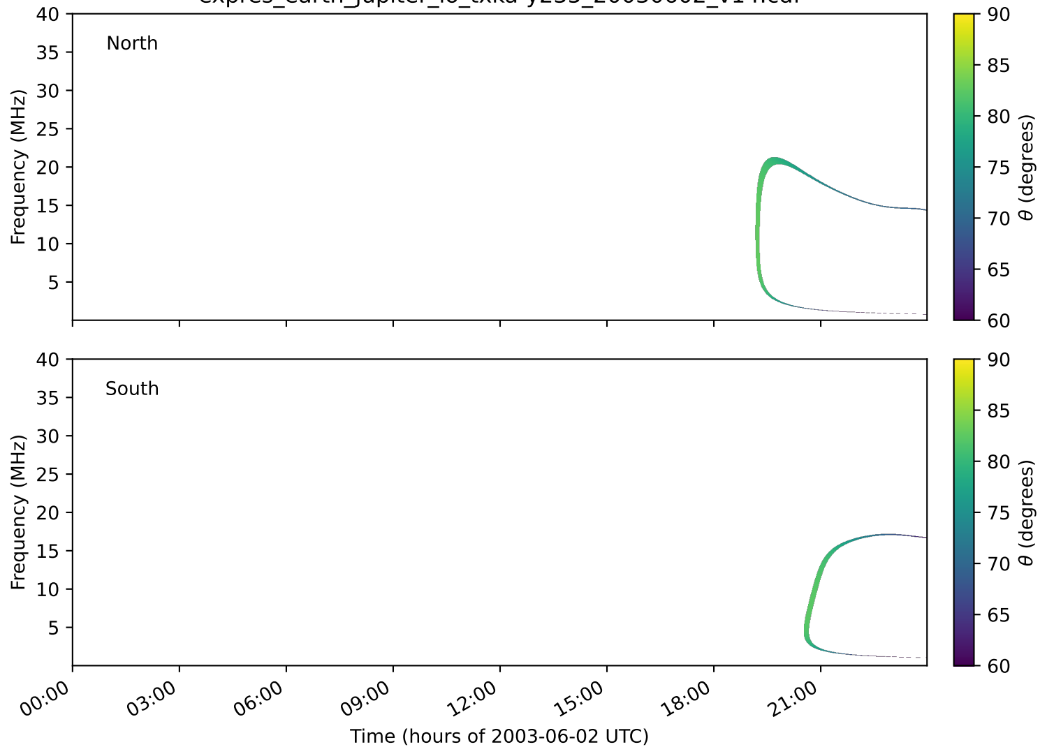
expres_earth_jupiter_io_txka-y235_20030602_v14.cdf
