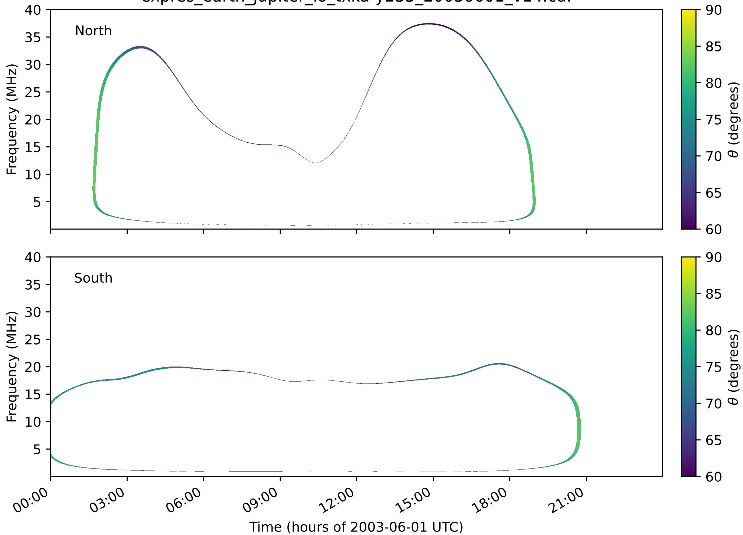
expres_earth_jupiter_io_txka-y235_20030601_v14.cdf
