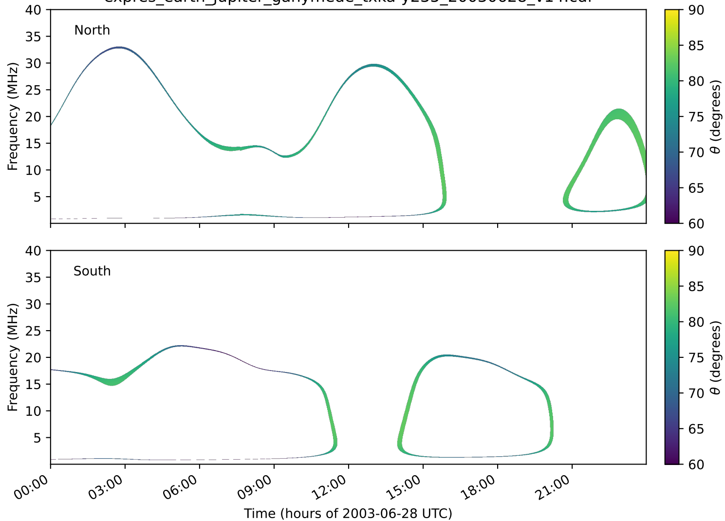
expres_earth_jupiter_ganymede_txka-y235_20030628_v14.cdf
