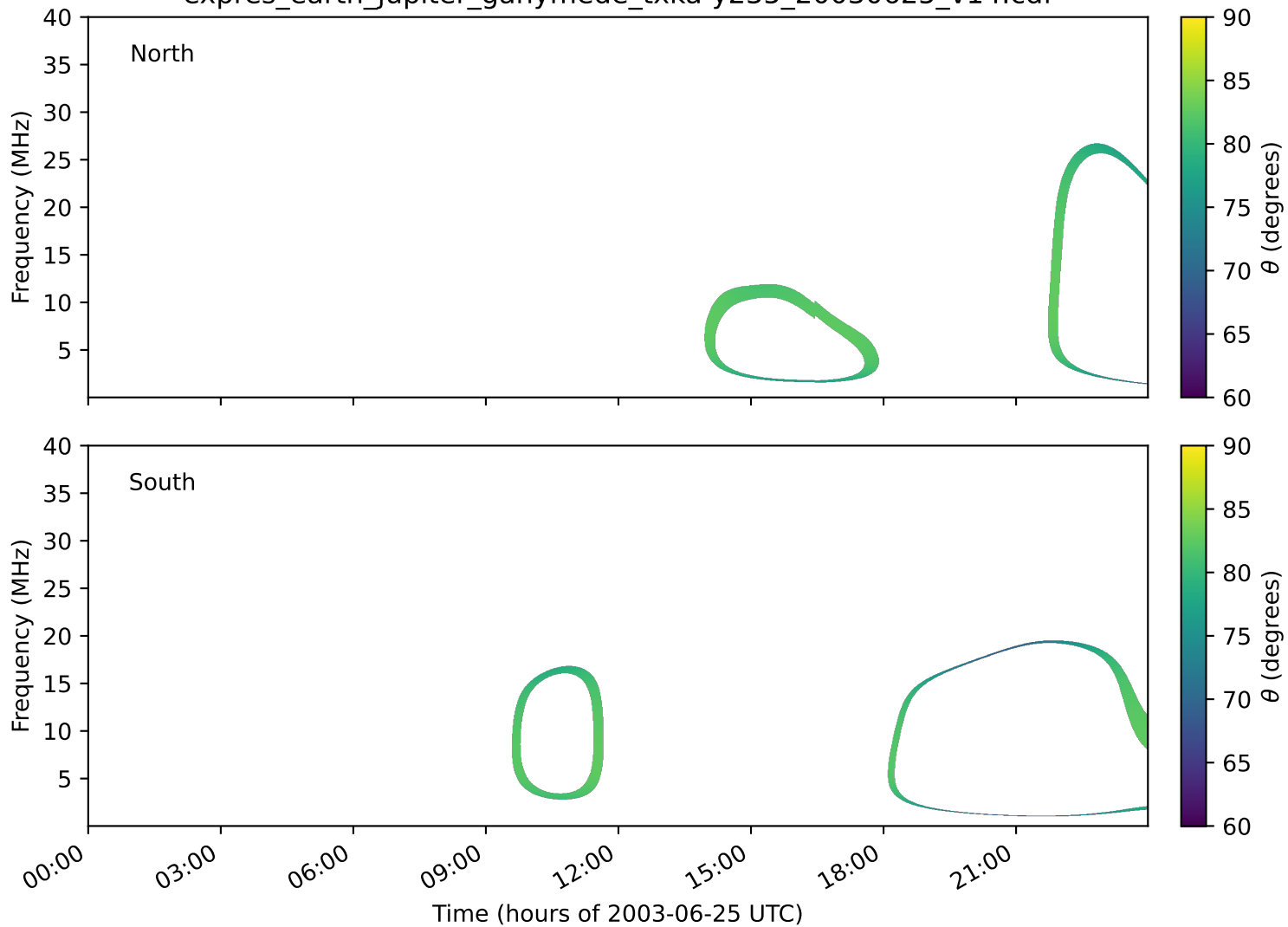
expres_earth_jupiter_ganymede_txka-y235_20030625_v14.cdf
