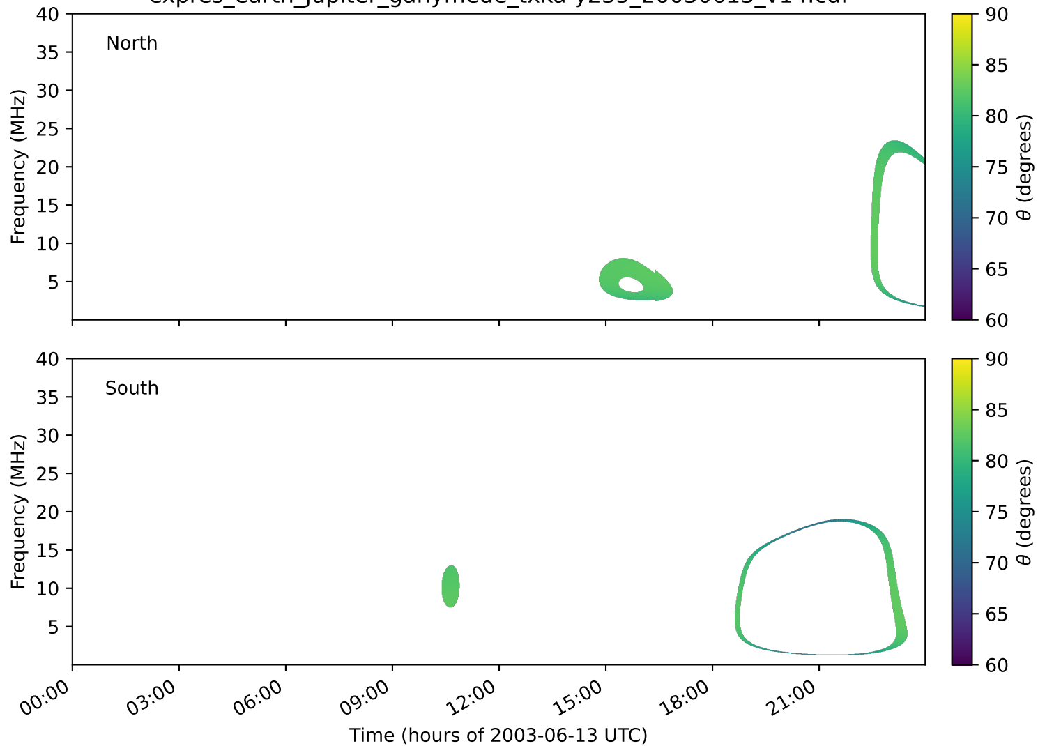
expres_earth_jupiter_ganymede_txka-y235_20030613_v14.cdf
