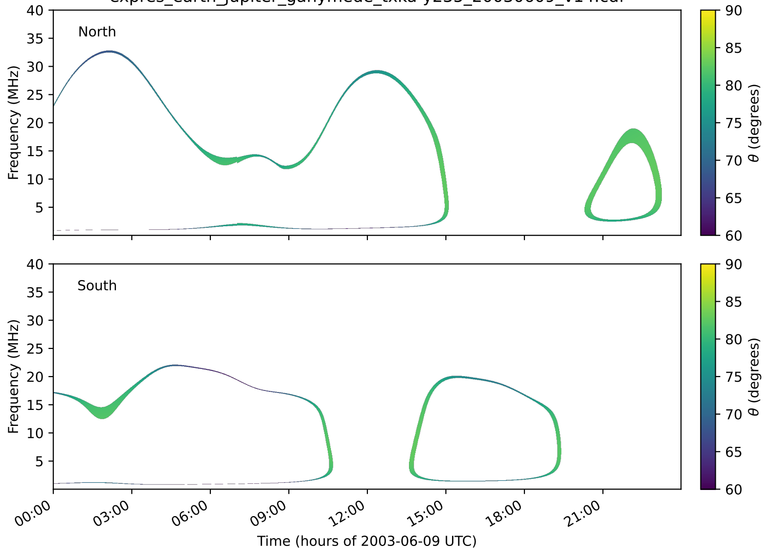
expres_earth_jupiter_ganymede_txka-y235_20030609_v14.cdf
