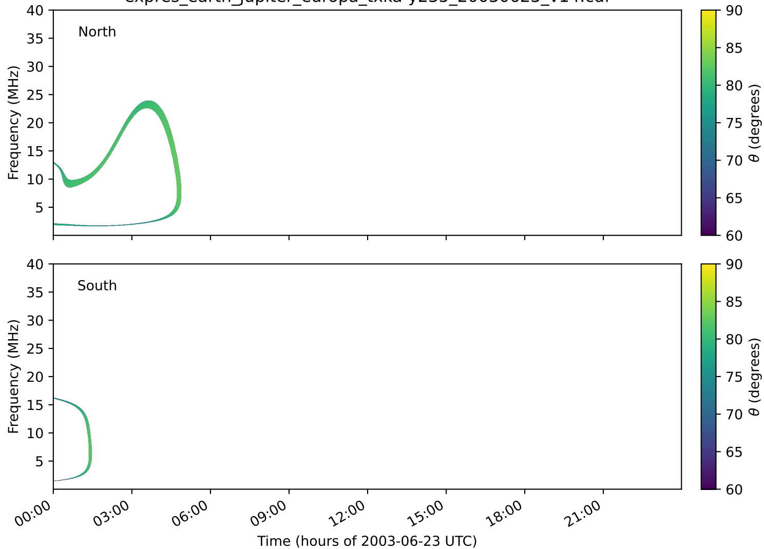
expres_earth_jupiter_europa_txka-y235_20030623_v14.cdf
