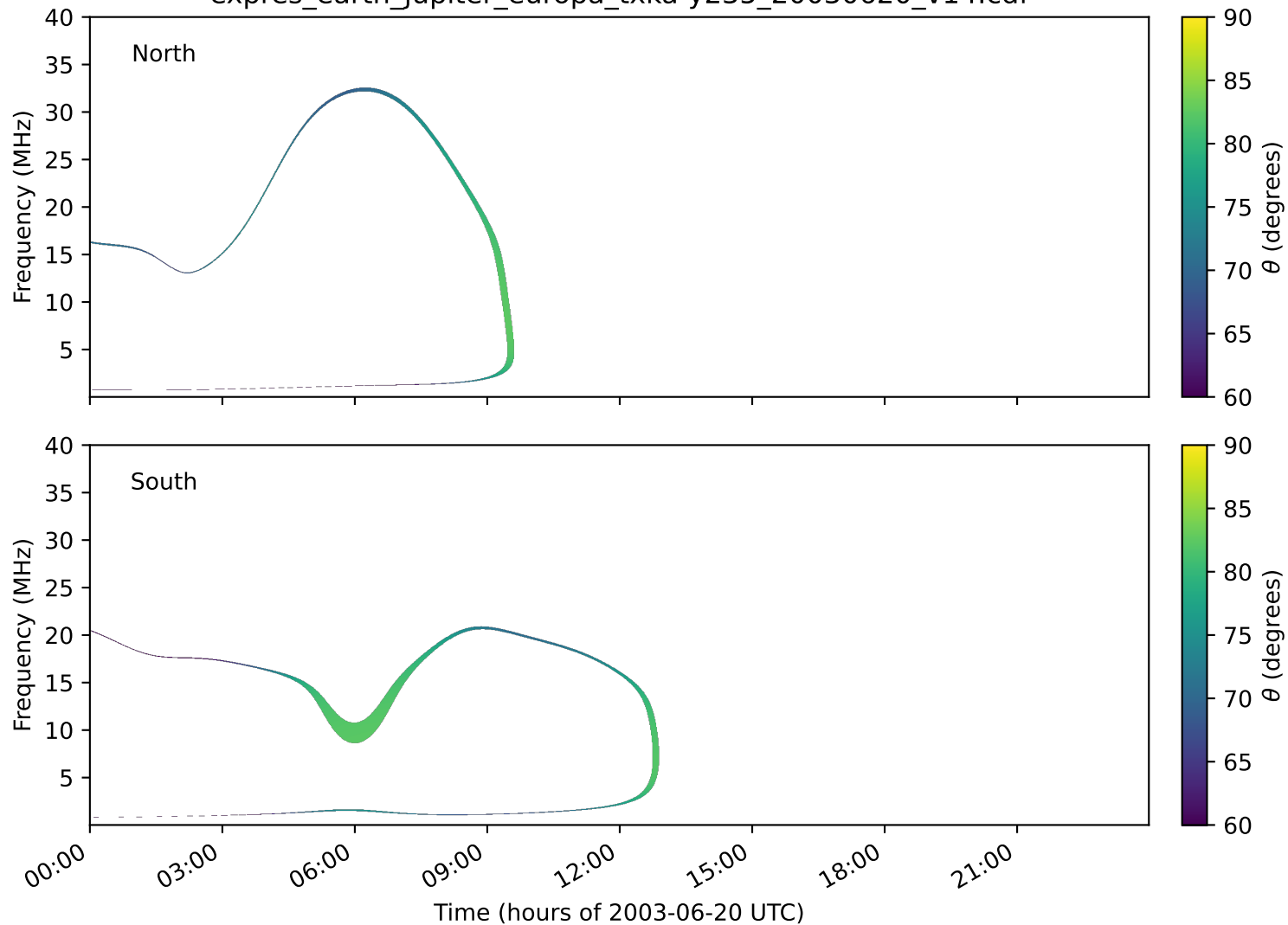
expres_earth_jupiter_europa_txka-y235_20030620_v14.cdf
