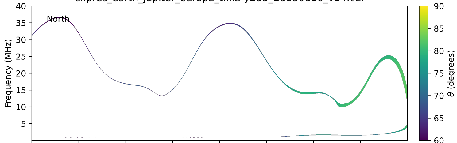
expres_earth_jupiter_europa_txka-y235_20030616_v14.cdf
