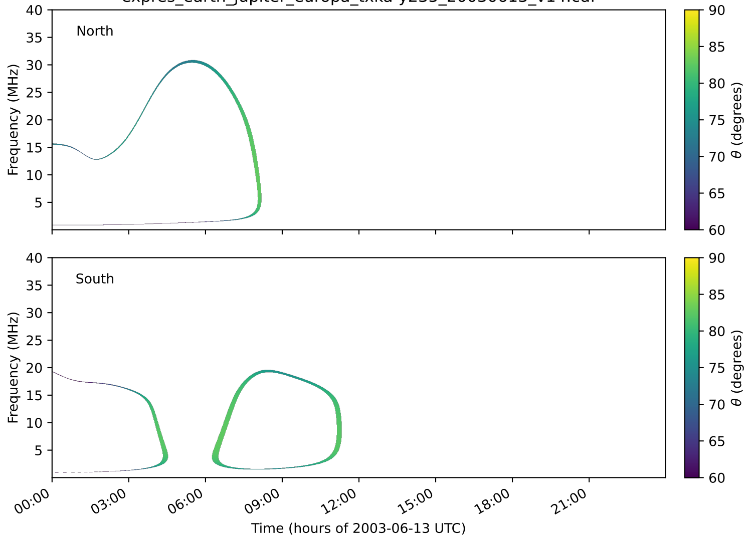
expres_earth_jupiter_europa_txka-y235_20030613_v14.cdf
