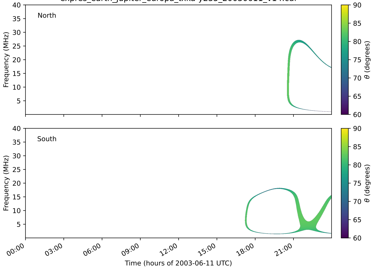
expres_earth_jupiter_europa_txka-y235_20030611_v14.cdf
