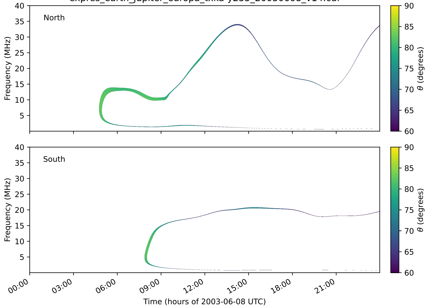
expres_earth_jupiter_europa_txka-y235_20030608_v14.cdf
