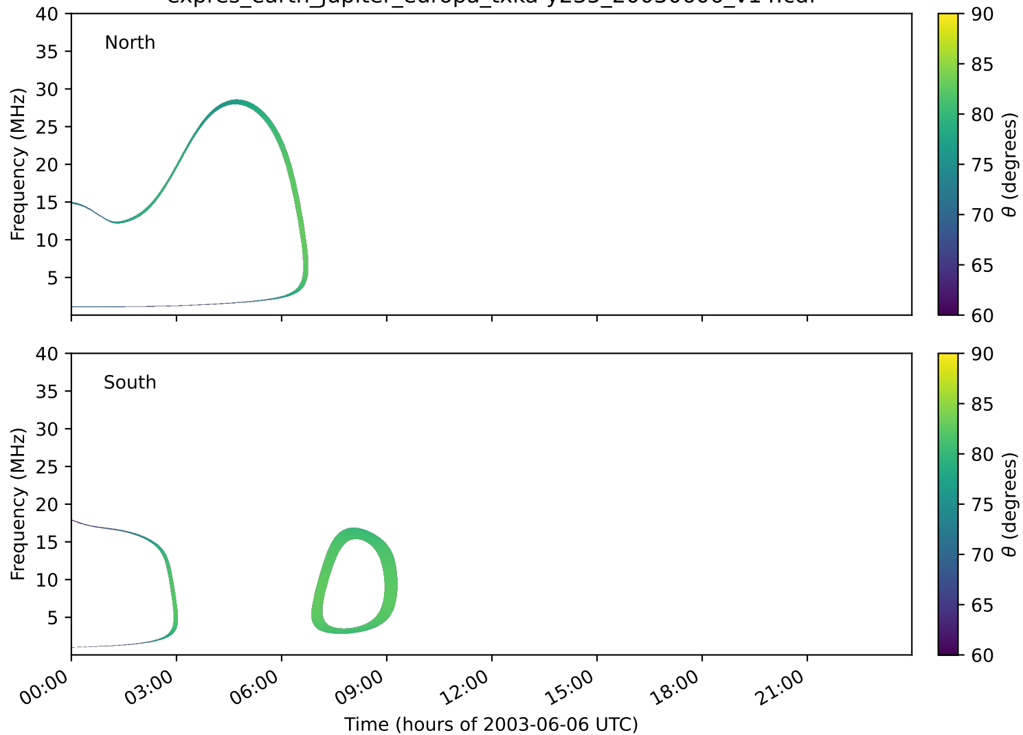
expres_earth_jupiter_europa_txka-y235_20030606_v14.cdf
