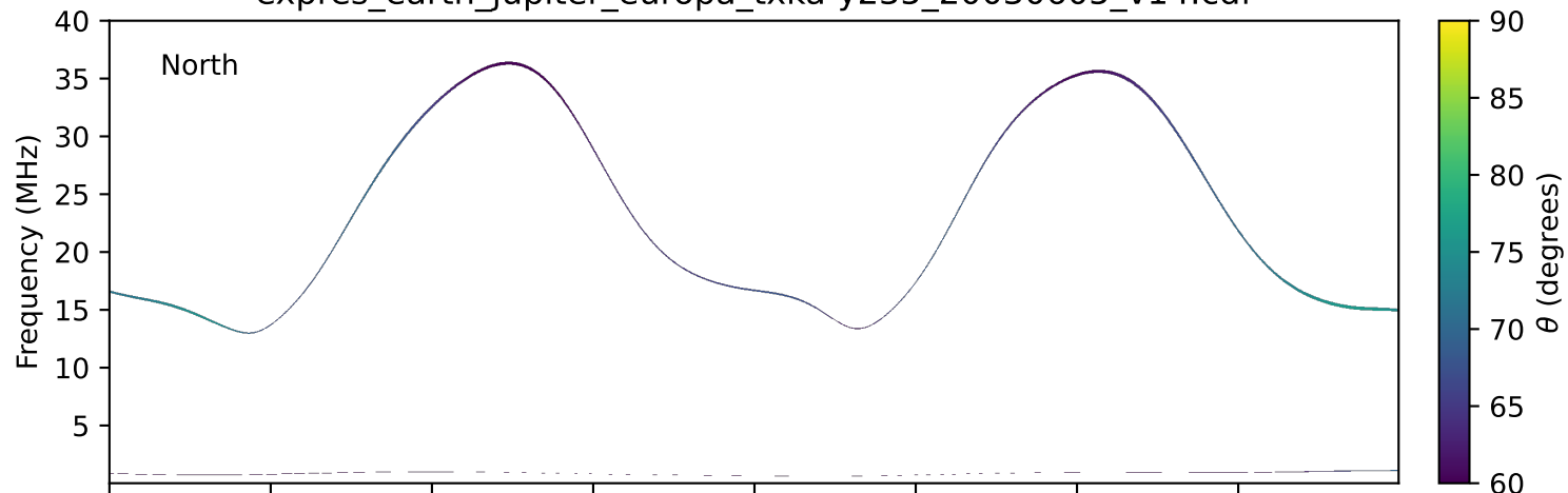
expres_earth_jupiter_europa_txka-y235_20030605_v14.cdf
