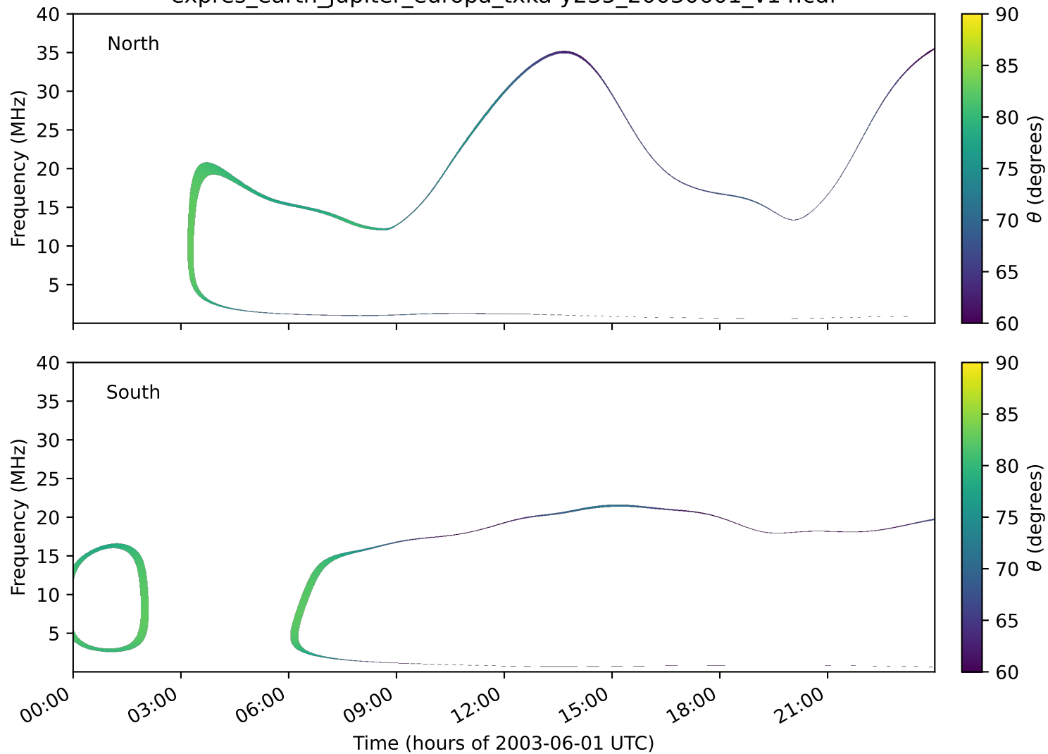
expres_earth_jupiter_europa_txka-y235_20030601_v14.cdf
