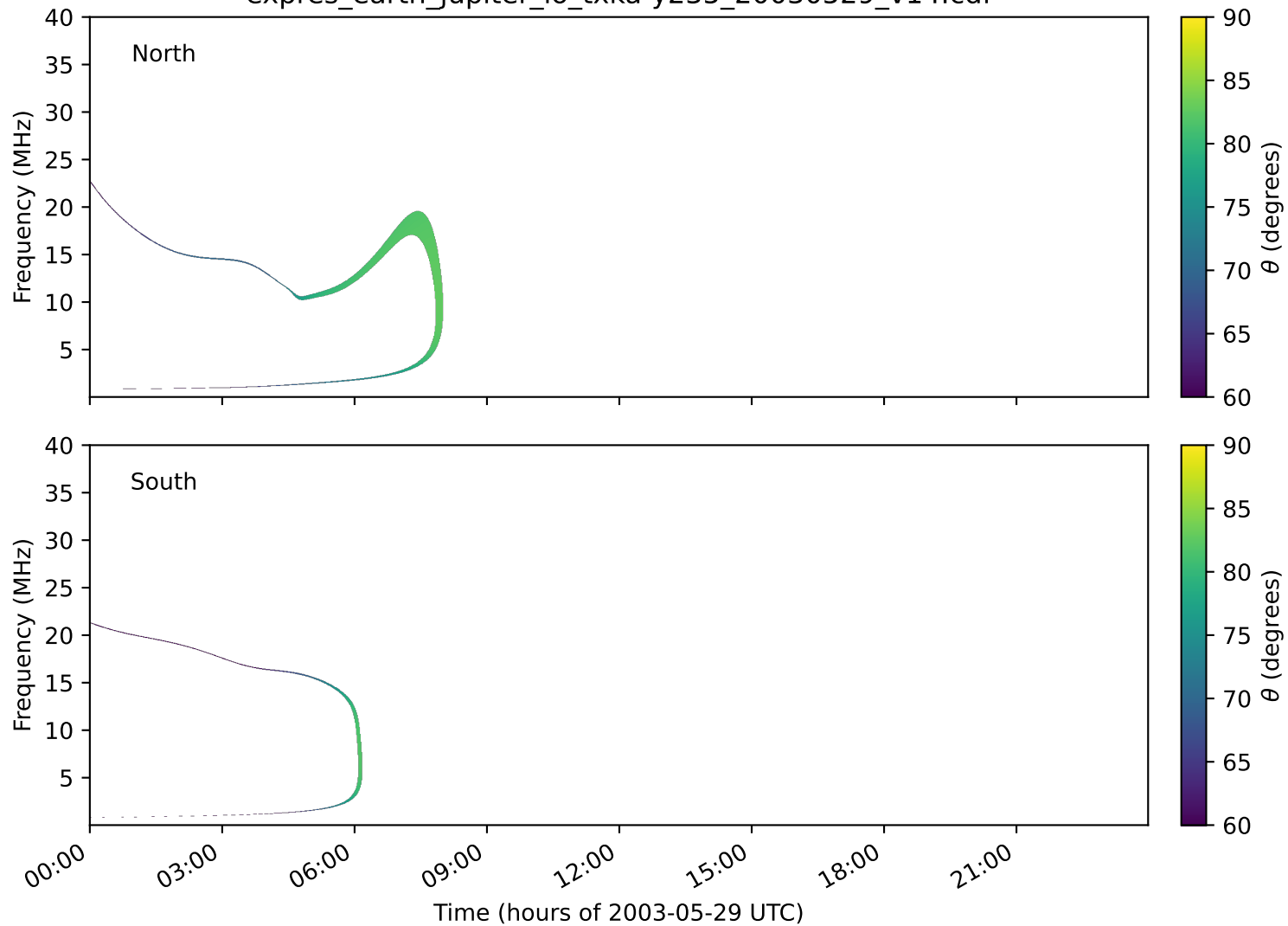
expres_earth_jupiter_io_txka-y235_20030529_v14.cdf
