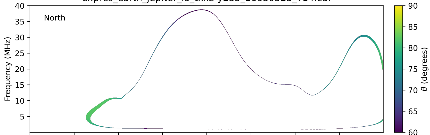
expres_earth_jupiter_io_txka-y235_20030523_v14.cdf
