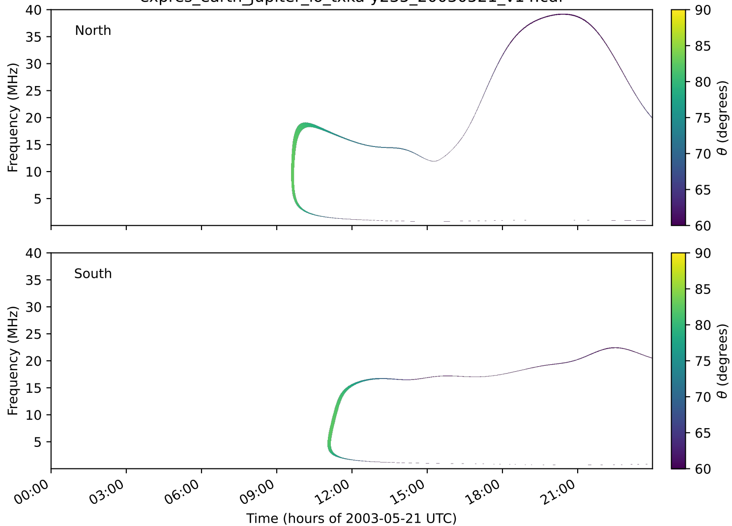
expres_earth_jupiter_io_txka-y235_20030521_v14.cdf
