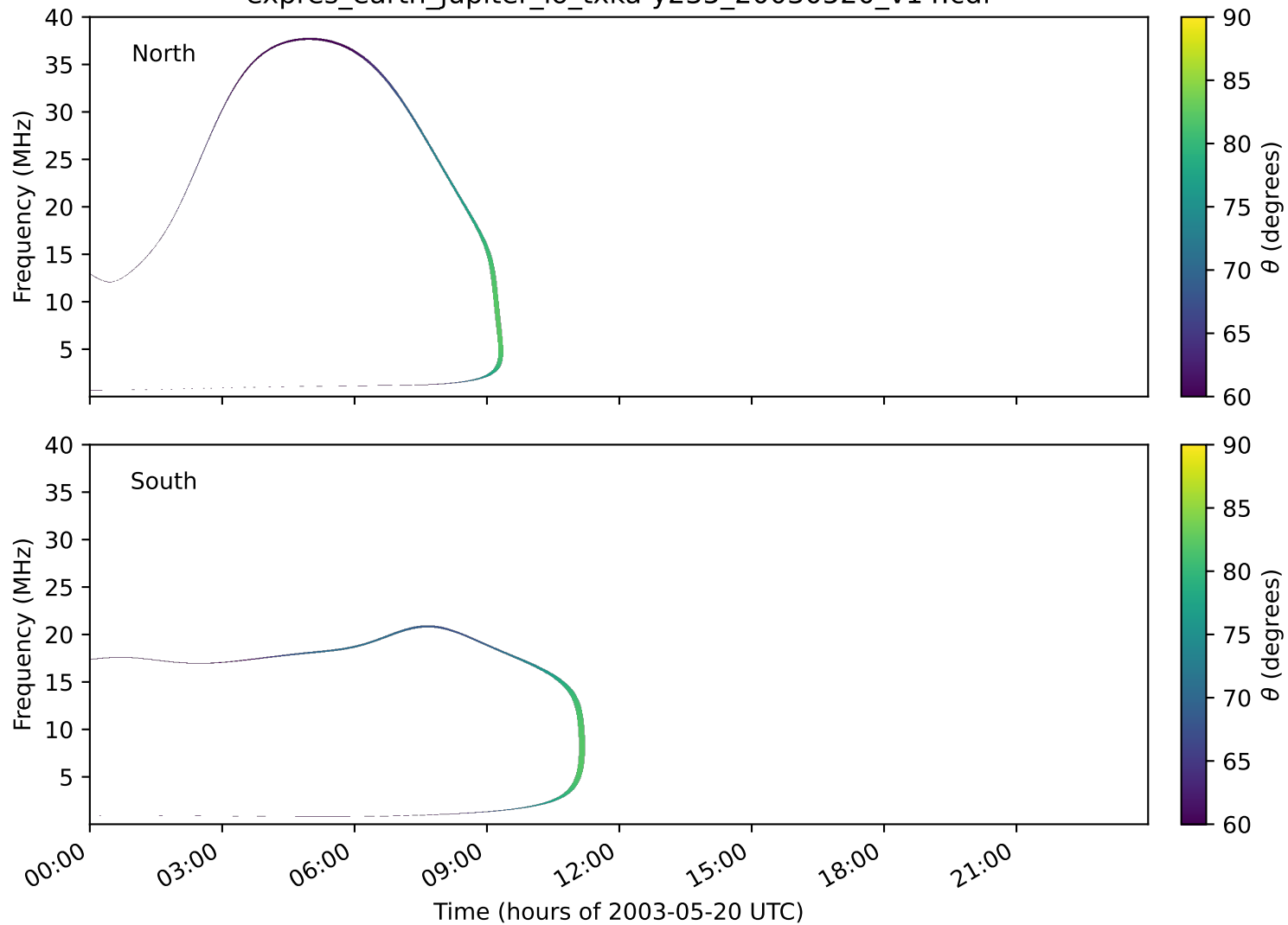
expres_earth_jupiter_io_txka-y235_20030520_v14.cdf
